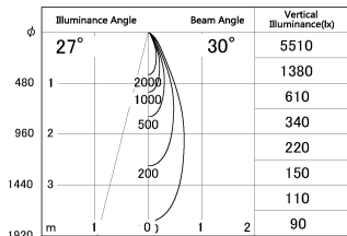
■ Direct Horizontal Illuminance SD287-0635BHC40-DMWL
