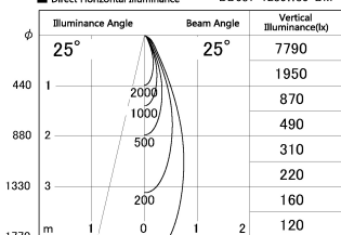
■ Direct Horizontal Illuminance DD087-1230W30-DM
