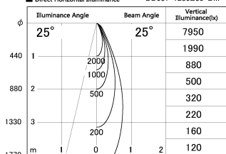
■ Direct Horizontal Illuminance DD087-1230B35-DM
