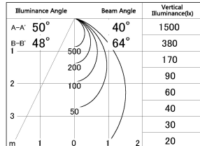
■ Direct Horizontal Illuminance DD154-08MB9030
