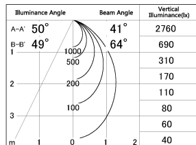
■ Direct Horizontal Illuminance DD154-15MB9035
