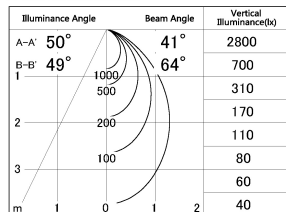
■ Direct Horizontal Illuminance DD154-15MB9040
