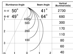
■ Direct Horizontal Illuminance DD154-15MW9027-DM
