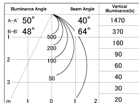
■ Direct Horizontal Illuminance DD154-08MW9027-DM
