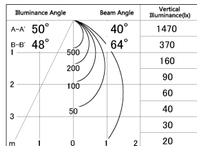
■ Direct Horizontal Illuminance DD154-08MB9027-DM
