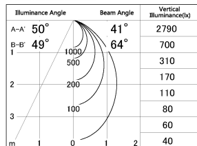
■ Direct Horizontal Illuminance DD154-15MW9030-DM
