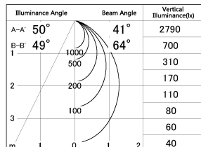
■ Direct Horizontal Illuminance DD154-15MB9030-DM
