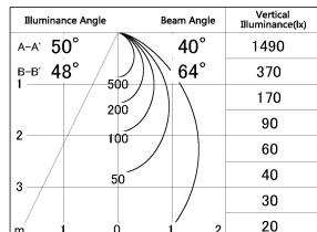
■ Direct Horizontal Illuminance DD154-08MB9035-DM
