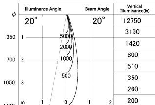
■ Direct Horizontal Illuminance DD187-0625W9027
