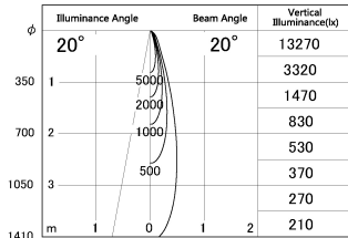
■ Direct Horizontal Illuminance DD187-0625W9030
