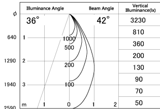
■ Direct Horizontal Illuminance DD187-0650W9030
