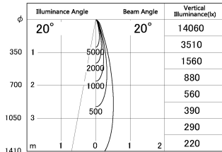
■ Direct Horizontal Illuminance DD187-0625W9040
