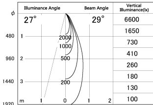
■ Direct Horizontal Illuminance DD187-0635W9040
