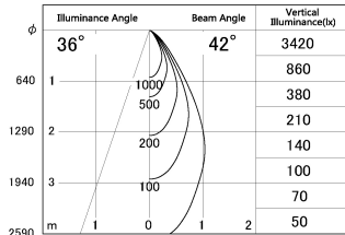
■ Direct Horizontal Illuminance DD187-0650W9040
