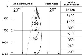
■ Direct Horizontal Illuminance DD187-0625B9027
