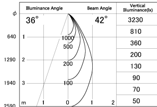
■ Direct Horizontal Illuminance DD187-0650B9030
