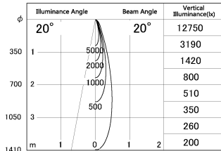
■ Direct Horizontal Illuminance DD187-0625W9027-DM1
