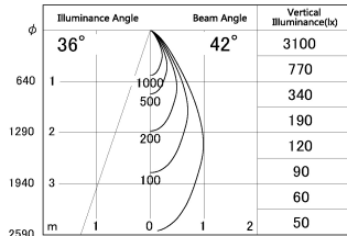
■ Direct Horizontal Illuminance DD187-0650W9027-DM1
