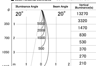
■ Direct Horizontal Illuminance DD187-0625W9030-DM1
