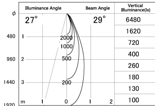
■ Direct Horizontal Illuminance DD187-0635W9035-DM1
