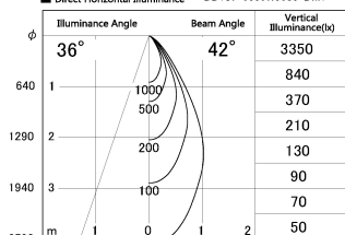
■ Direct Horizontal Illuminance DD187-0650W9035-DM1
