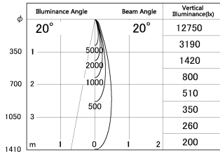
■ Direct Horizontal Illuminance DD187-0625B9027-DM1
