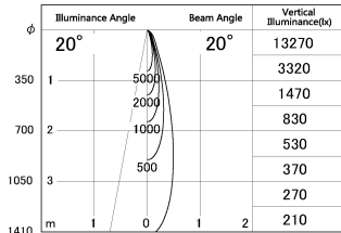
■ Direct Horizontal Illuminance DD187-0625B9030-DM1
