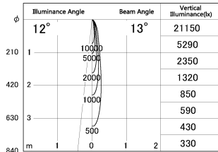
■ Direct Horizontal Illuminance DD187-0615B9035-DM1
