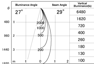
■ Direct Horizontal Illuminance DD187-0635B9035-DM1
