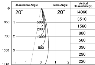
■ Direct Horizontal Illuminance DD187-0625B9040-DM1
