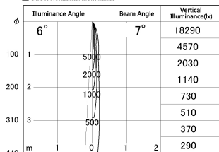
■ Direct Horizontal Illuminance DD130-0504BW9027-DM1
