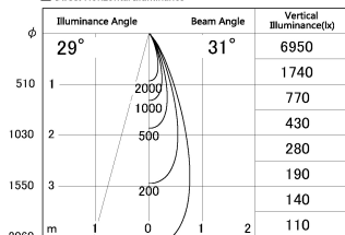
■ Direct Horizontal Illuminance DD130-0535BW9027-DM1
