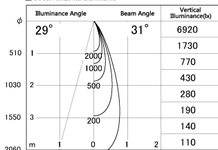
■ Direct Horizontal Illuminance DD130-0535MB9027-DM1
