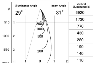
■ Direct Horizontal Illuminance DD130-0535MW9027-DM1
