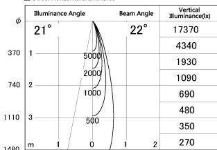
■ Direct Horizontal Illuminance DD130-1225MB9027-DM1
