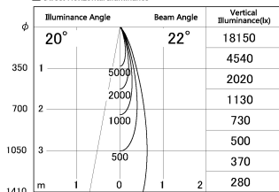
■ Direct Horizontal Illuminance DD130-1225WB9027-DM1
