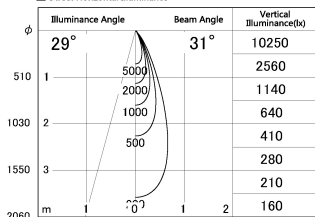
■ Direct Horizontal Illuminance DD130-1235MB9027-DM1
