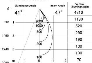
■ Direct Horizontal Illuminance DD130-1250MW9027-DM1
