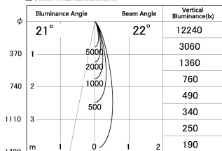
■ Direct Horizontal Illuminance DD130-0525MW9030-DM1
