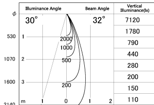
■ Direct Horizontal Illuminance DD130-0535WB9030-DM1
