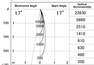
■ Direct Horizontal Illuminance DD130-1215MB9030-DM1
