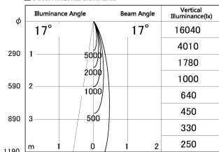
■ Direct Horizontal Illuminance DD130-0515MB9035-DM1
