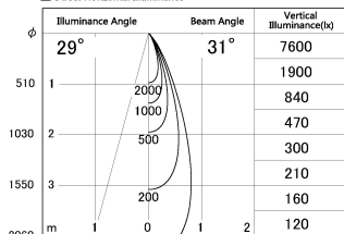
■ Direct Horizontal Illuminance DD130-0535BW9035-DM1
