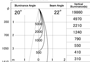
■ Direct Horizontal Illuminance DD130-1225WB9035-DM1
