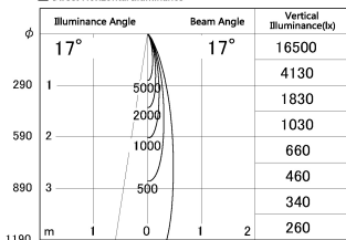
■ Direct Horizontal Illuminance DD130-0515MB9040-DM1
