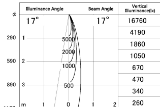
■ Direct Horizontal Illuminance DD130-0515WB9040-DM1
