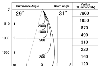
■ Direct Horizontal Illuminance DD130-0535MW9040-DM1
