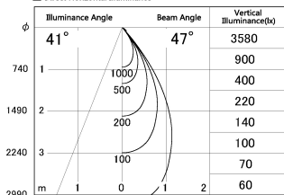
■ Direct Horizontal Illuminance DD130-0550MB9040-DM1
