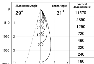
■ Direct Horizontal Illuminance DD130-1235BW9040-DM1
