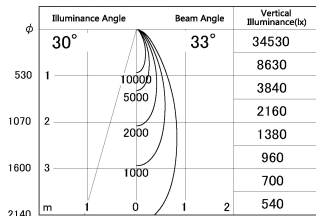
■ Direct Horizontal Illuminance DD126-4035W9027-LX
